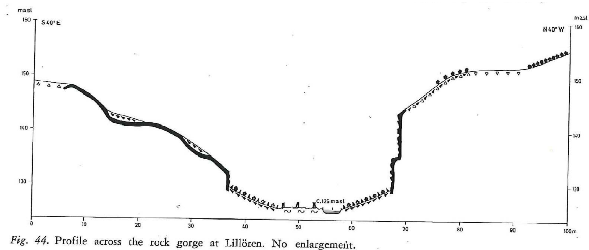
Figur 1. Figuren visar ravinens profil (Agrell, 1974).
